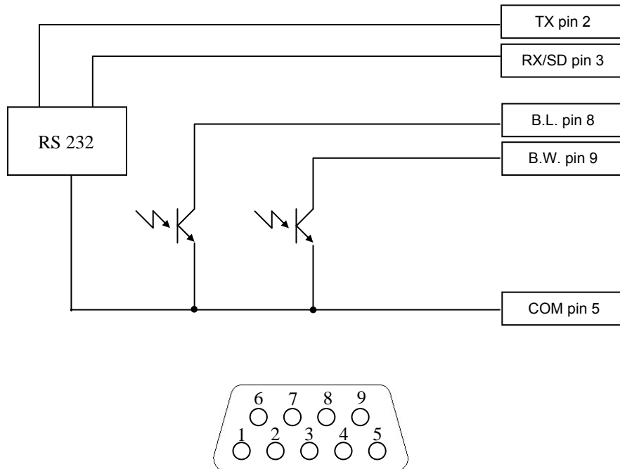
Sub D 9-pin female (computer interface) connector
